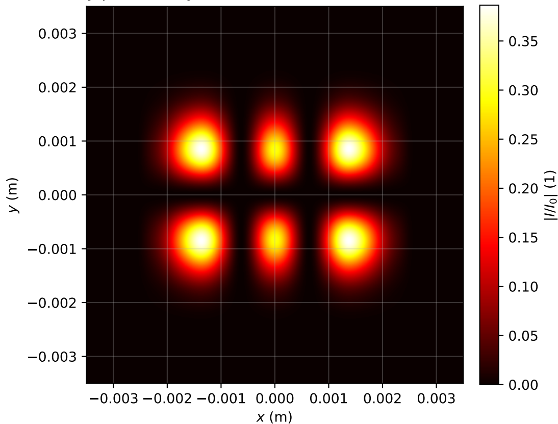
Intensity profile I(x, y, z = 2.866)/I_0 , P_{in}=1.0P_{cr} , artificial time
